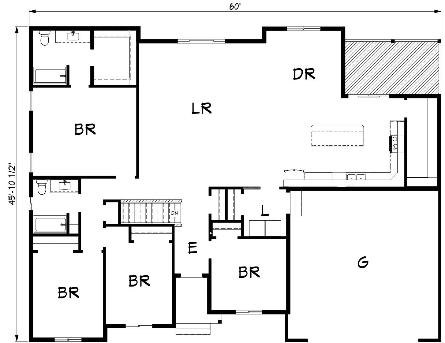
1st Floorplan
