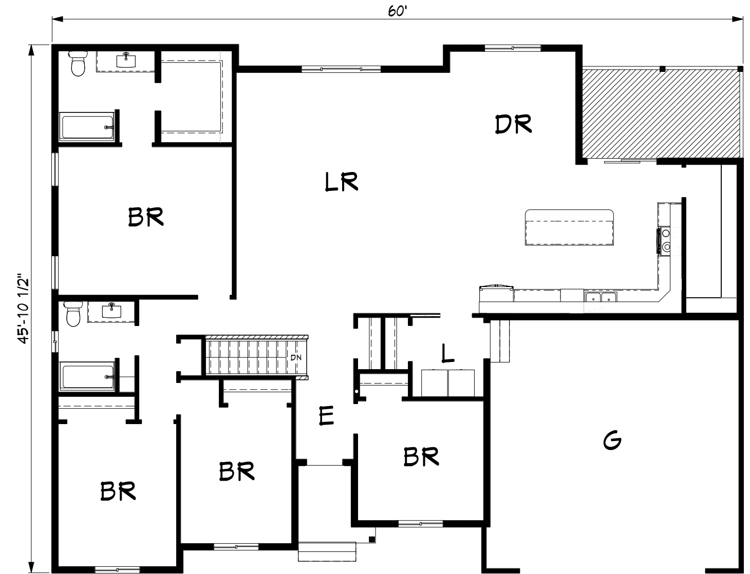
1st Floorplan
