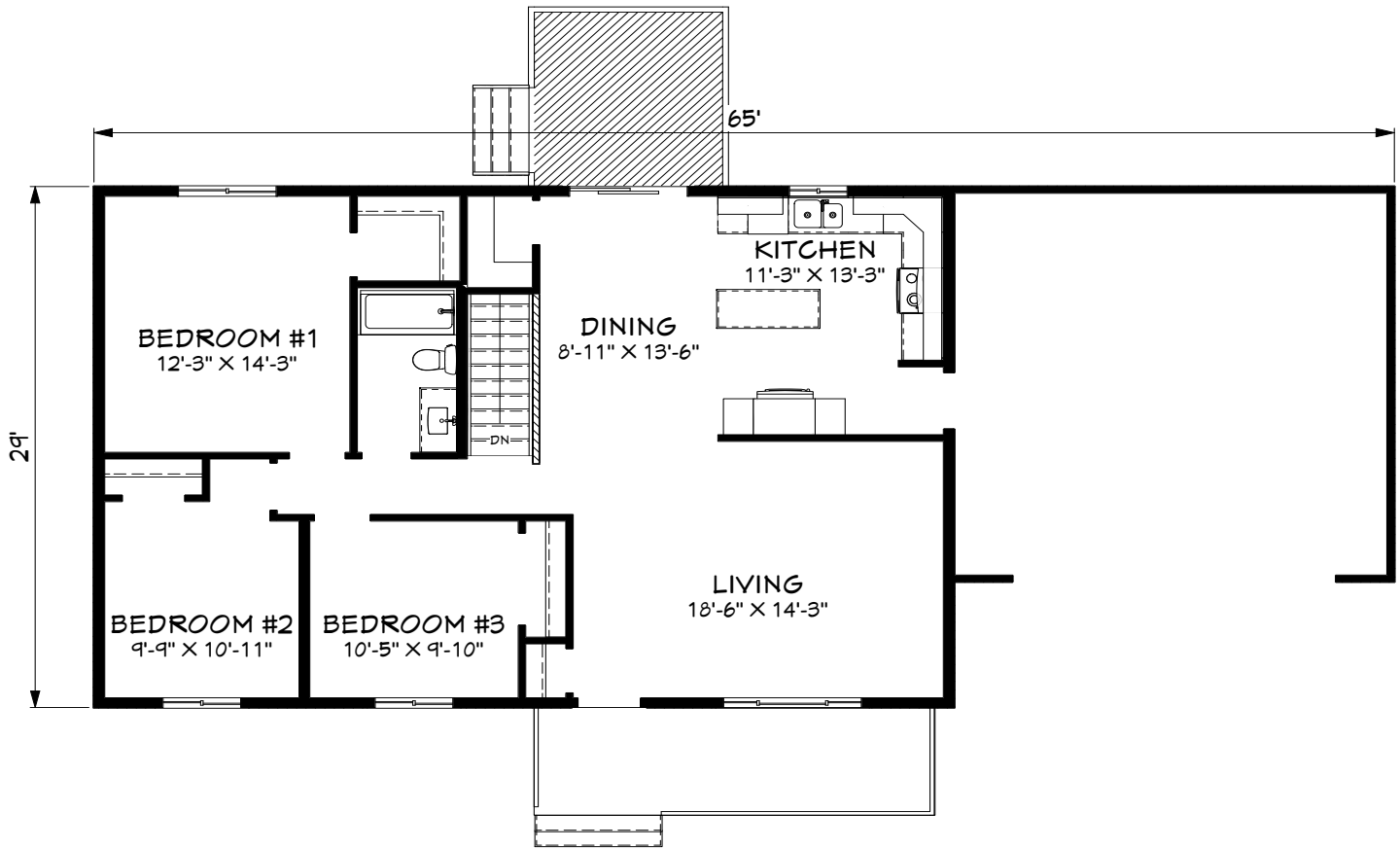
1st Floorplan
