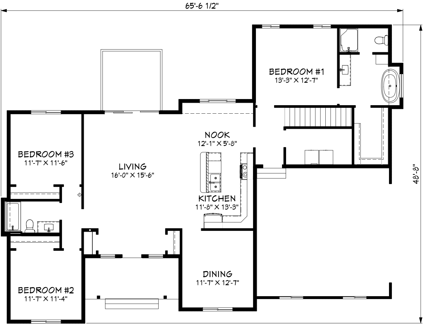
1st Floorplan
