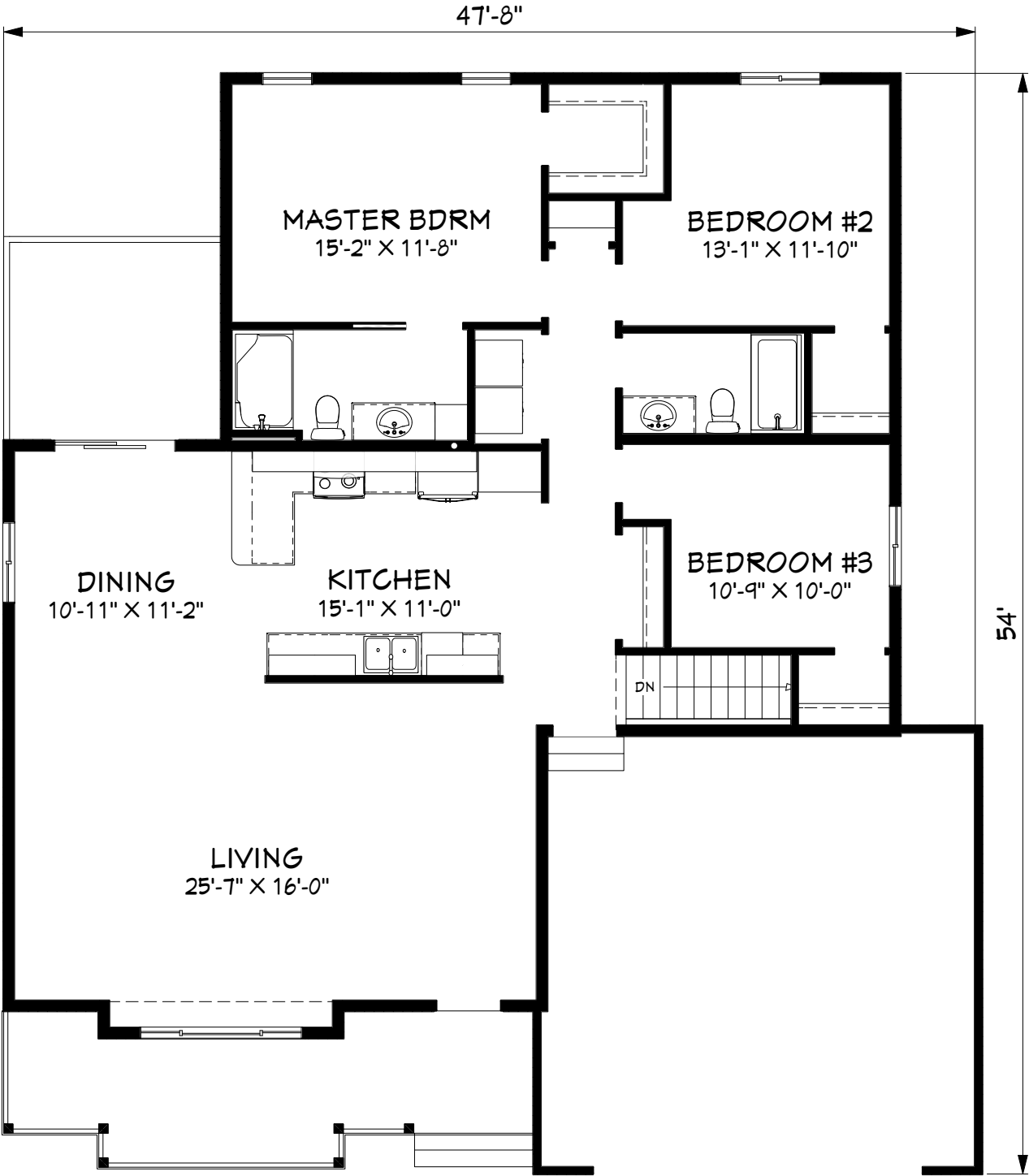
1st Floorplan
